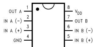
Figure 3. Top View SOIC & VSSOP Package See Package Number D0008A, DGK0008A
