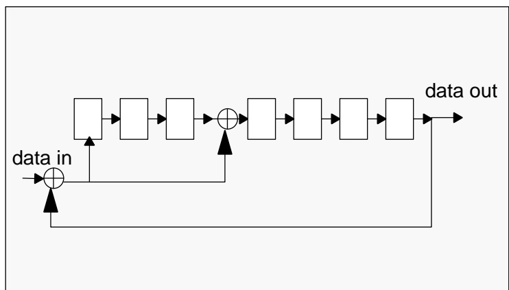
Figure 4-20: CRC7 Generator/Checker
