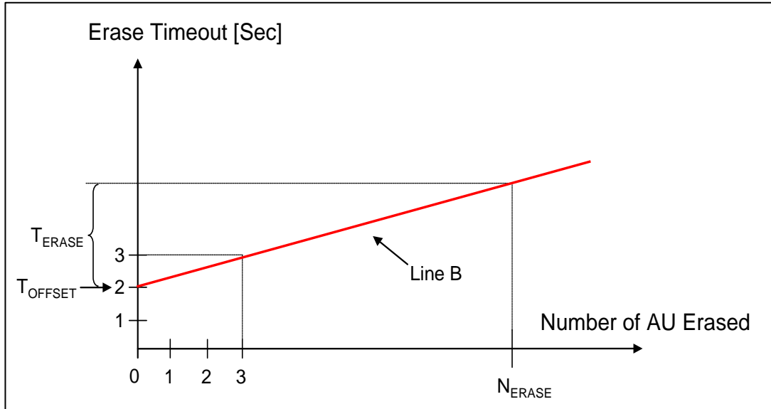
Figure 4-57: Example Erase Characteristics (Case 2 TOFFSET=2)
